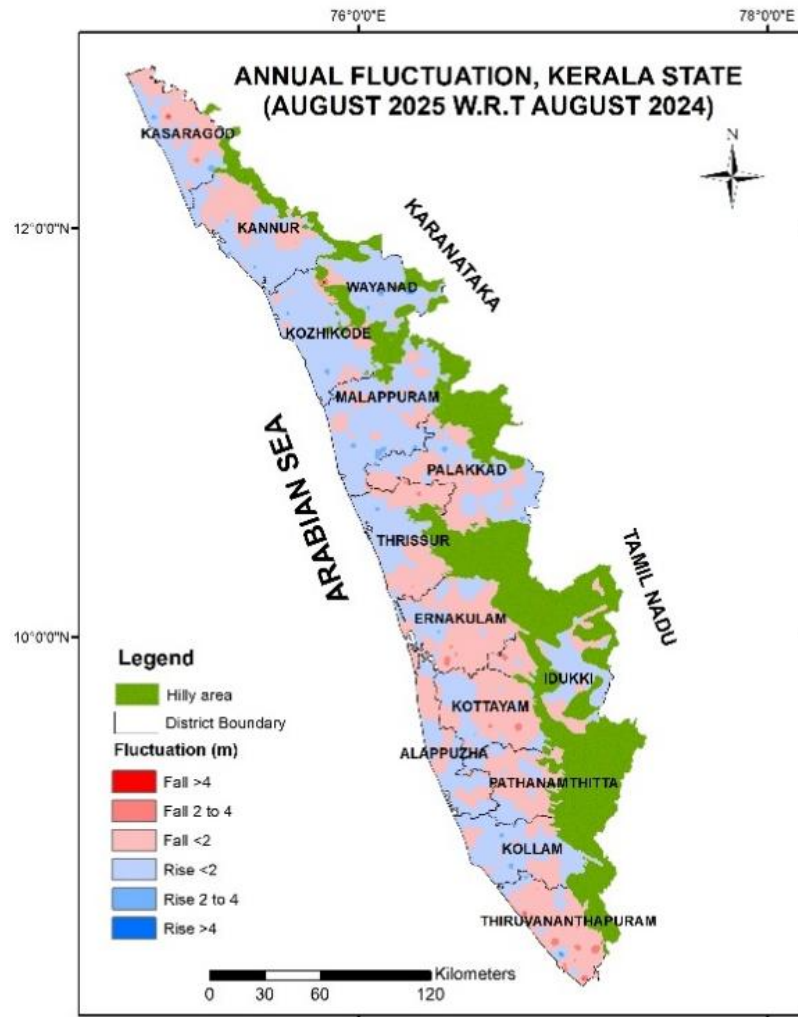
Figure-10: Annual water level fluctuation in unconfined aquifer (August 2024 to August 2025)
