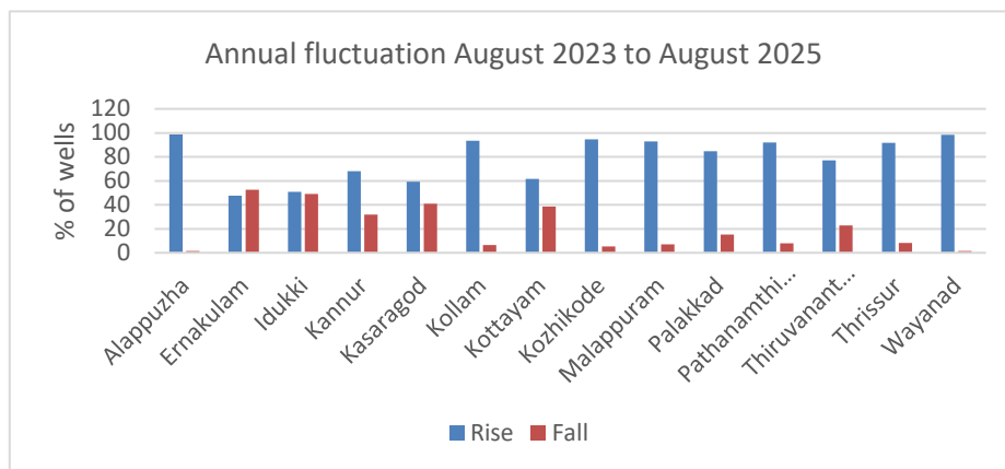
Figure-7: Percentage of wells showing rise and fall in WL in unconfined aquifer(August 2023 to August 2025)
