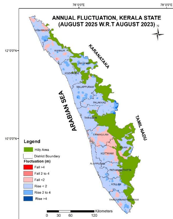
Figure-8: Annual water level fluctuation in unconfined aquifer (August 2023 to August 2025)
