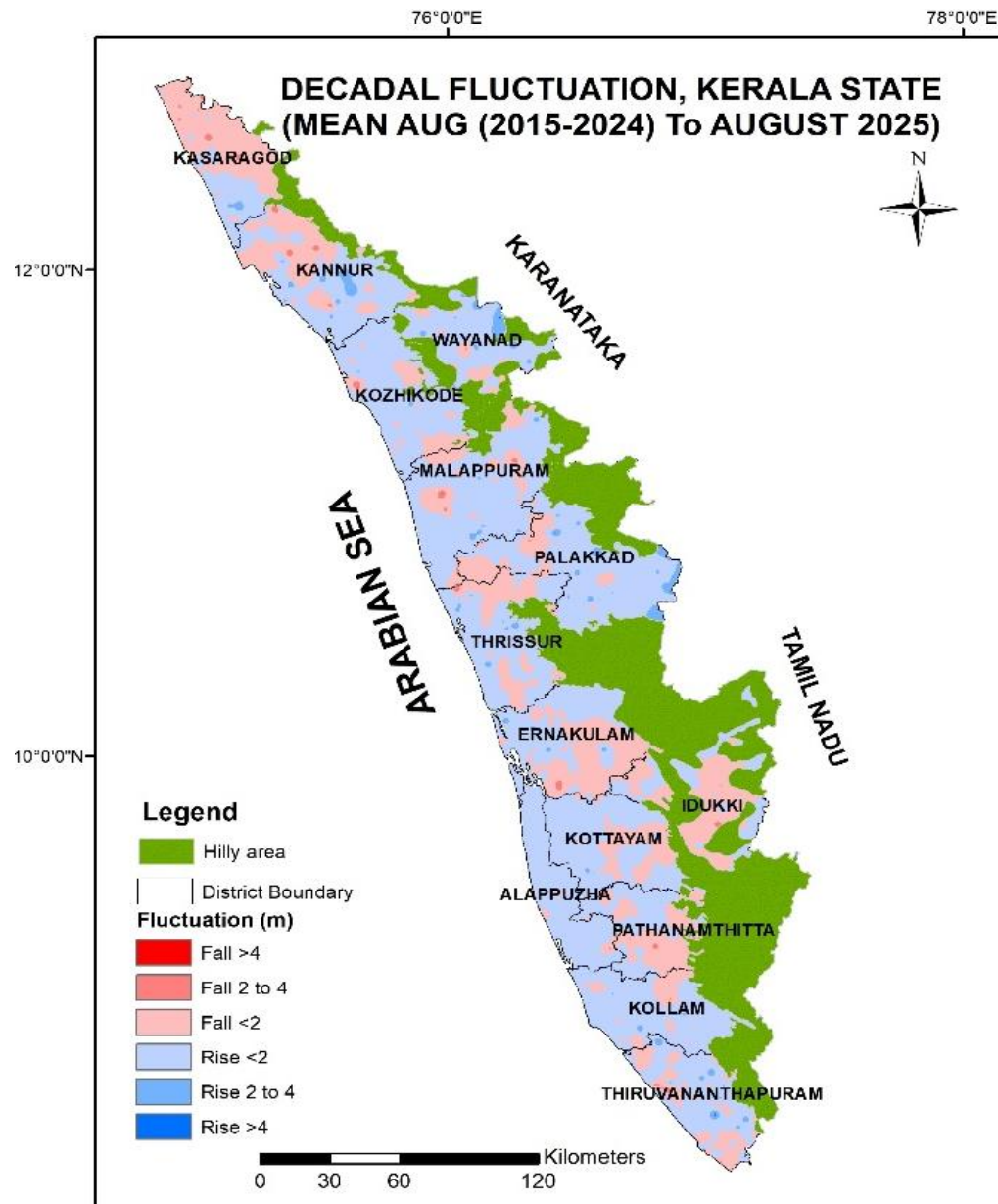
Figure-12: Water level fluctuation with respect to decadal mean (Aug (2015-2024) to Aug 2025)
