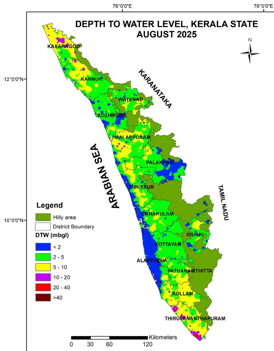
Figure-4: Depth to water Level in phreatic aquifer in Kerala during August 2025
