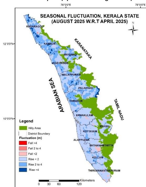
Figure-6: Seasonal water level fluctuation in unconfined aquifer (April 2025 to August 2025)
