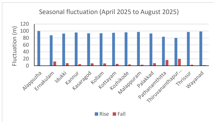
Figure-5: Percentage of wells showing rise and fall in WL in unconfined aquifer (April 2025 to August 2025)
