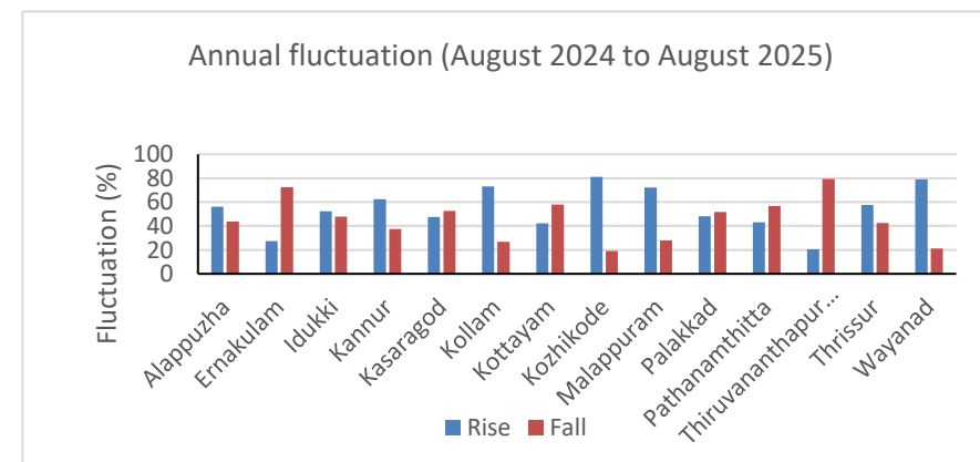
Figure-9: Percentage of wells showing rise and fall in WL
