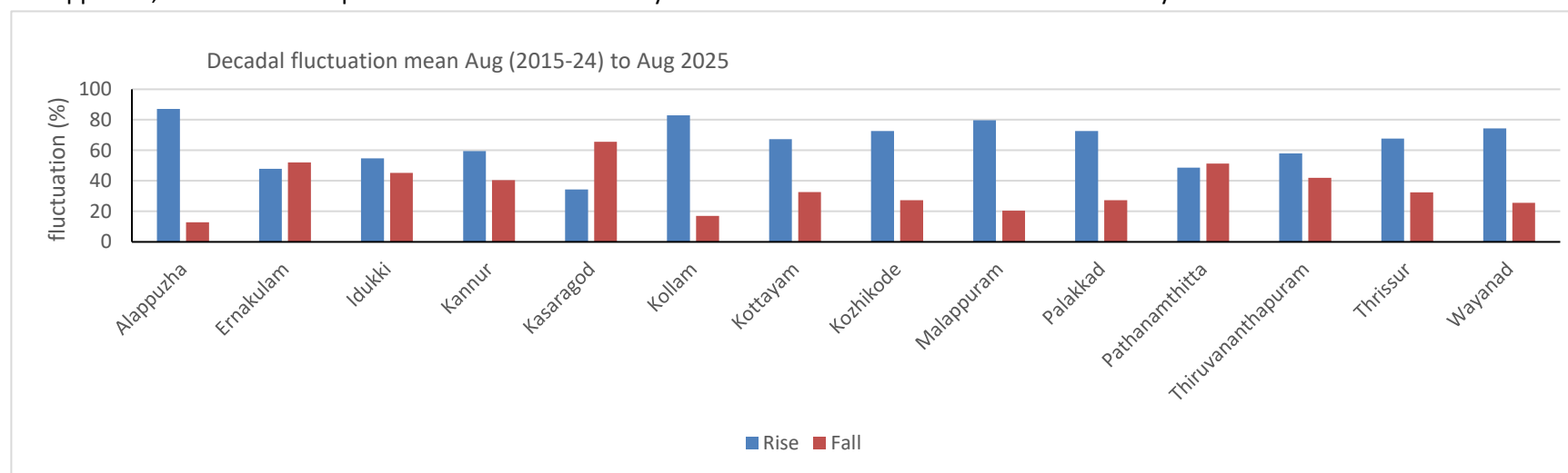
Figure-11: Percentage of wells showing rise and fall in WL in unconfined Aquifer(Decadal Mean August (2015-2024) to August 2025)
